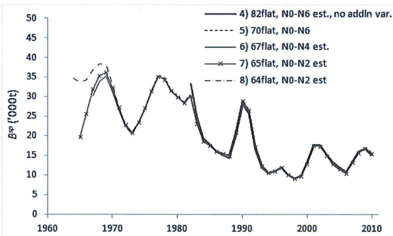
Fig. 3a: Spawning biomass trajectories cases 4 to 8.
