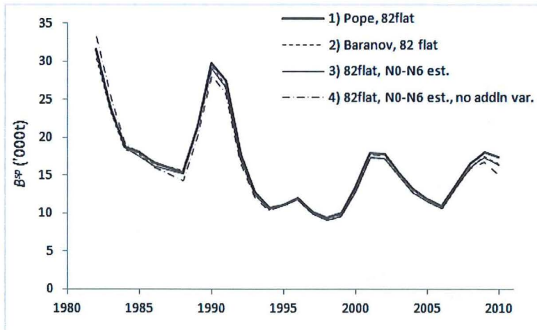
Fig. 1: Spawning biomass trajectories cases 1 to 4.
