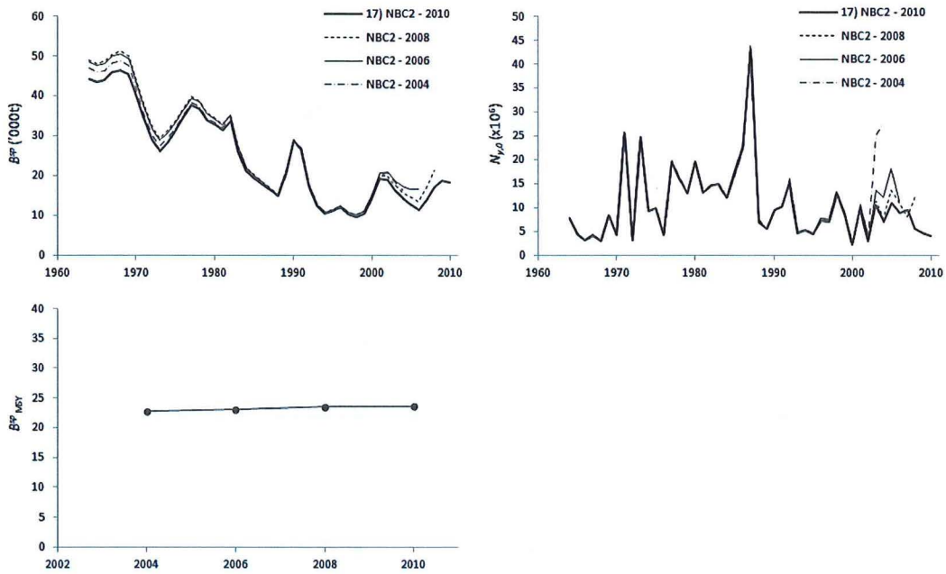
Fig. 17: Retrospective analysis for Case 17 (New Base Case 2), with a Ricker stock-recruitment function used in the estimation of B_{MSY}^{SP} .
